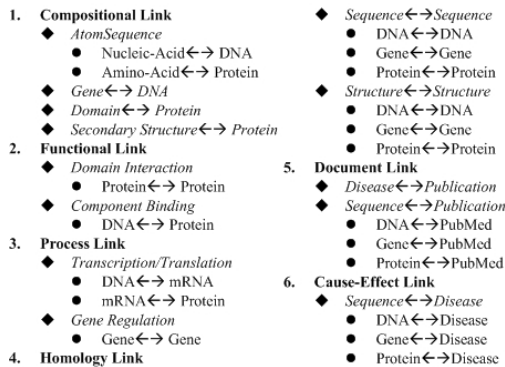
Fig. 3. Link Ontology
