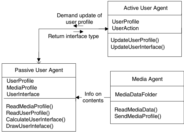
Fig. 3. Agents' model
