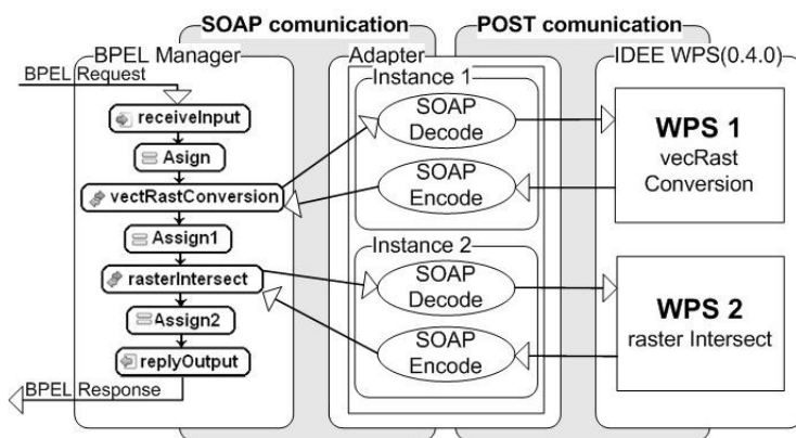
Fig. 6. BPEL's process
