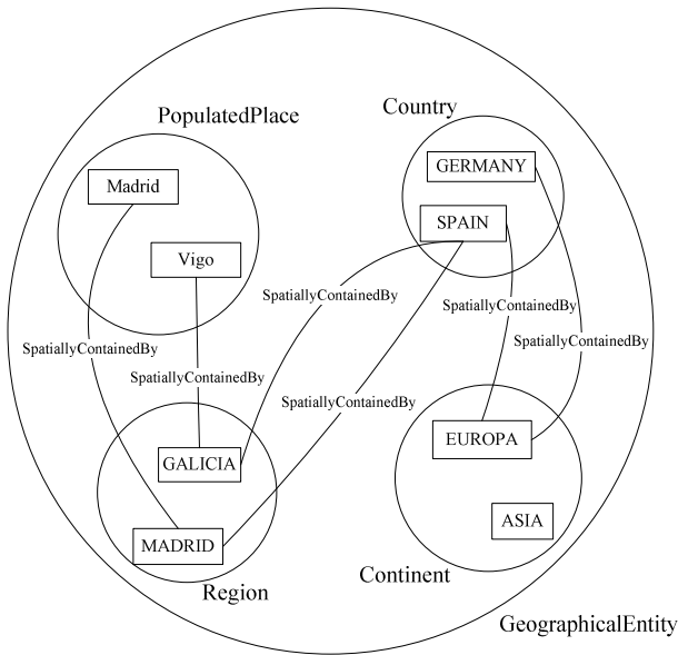
Fig. 1. Ontology instances
